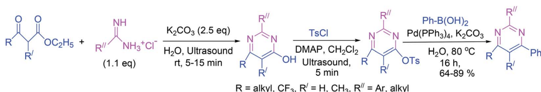
Scheme 16 Synthesis of 4-arylpurimides under ultrasound irradiation.
