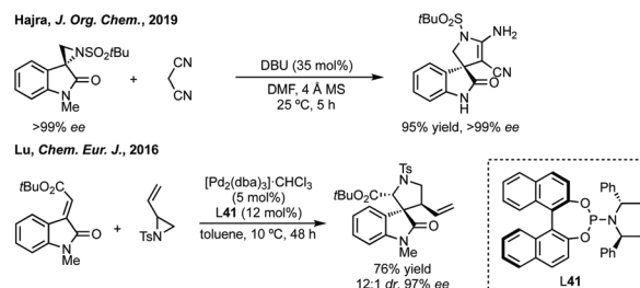
Scheme 41 3,3'-Spirocyproline oxindoles synthesised by aziridine ring expansion.
