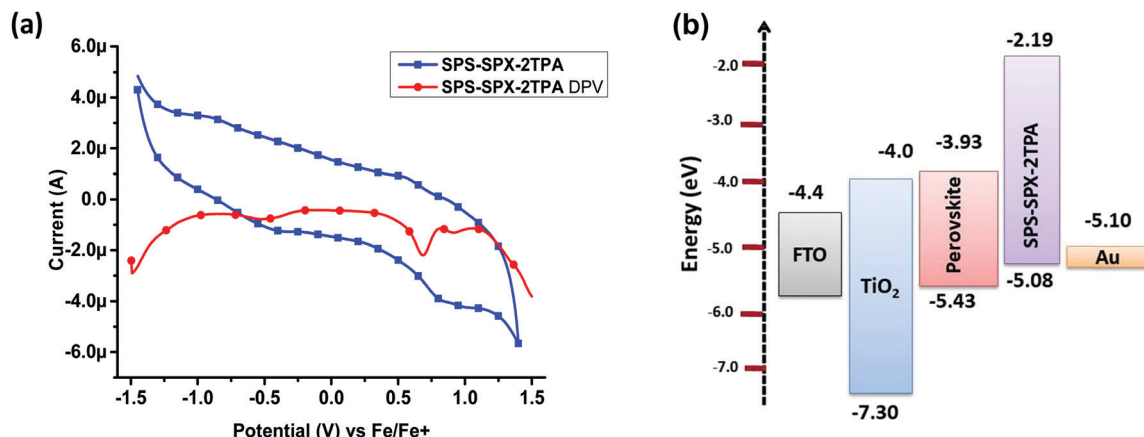
Fig. 3 (a) CV and DPV spectra of SPS-SPX-2TPA. (b) Energy level diagram of a PSC with SPS-SPX-2TPA as the HTM.
