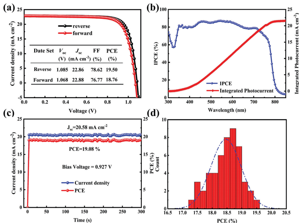
Fig. 3 (a) J - V curves of the champion FA 0.3 MA 0.7 PbI 3 -device under forward and reverse scan. (b) IPCE spectrum and the corresponding integrated J_{sc} . (c) The photo-current density and PCE with a given bias of 0.927 V. (d) Histograms of photovoltaic PCEs from 50 devices.
