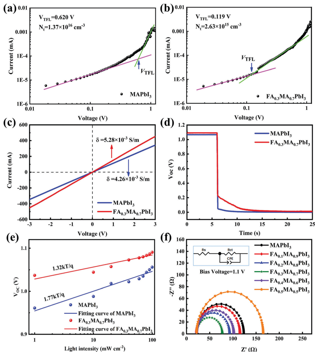
Fig. 4 Dark current–voltage curves of the electron-only devices for (a) MAPbI 3 and (b) FA 0.3 MA 0.7 PbI 3 , displaying a V TFL kink point behavior. (c) I – V curves of the devices with the structure of FTO/perovskite/Au for conductivity measurements. (d) OCVD curves of the MAPbI 3 -device and FA 0.3 MA 0.7 PbI 3 -device. (e) V oc values under different light intensities of the MAPbI 3 -device and FA 0.3 MA 0.7 PbI 3 -device. (f) The EIS of the champion devices based on the MAPbI 3 film and FA x MA 1-x PbI 3 films with different FA amounts.
