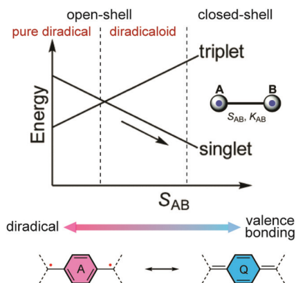
Fig. 2 Change of energies of triplet and singlet electron pairs with the increase in the one-electron overlap integral S_{AB} and resonances between open-shell diradical and closed-shell quinoid structures. Reproduced (adapted) from ref. 11 with permission from the Royal Society of Chemistry.
