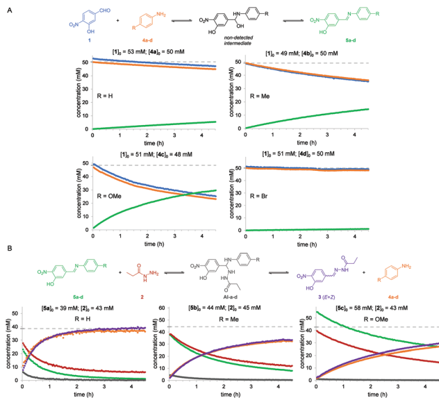
Fig. 3 (A) Reaction between aldehyde 1 and anilines 4a–d in CD 3 CN to form imines 5a–d . Plots show the concentrations (mM) of compounds 1 , 4a–d and 5a–d at different reaction times using approximately equal initial concentrations of reagents 1 and 4a–d . Grey dashed lines indicate the initial concentrations of the limiting reagents for each reaction. (B) Reaction between imines 5a–d and acylhydrazide 2 in CD 3 CN to form acylhydrazone 3 as a mixture of Z/E isomers. Plots show the concentrations (mM) of compounds 4a–c , 3 and 5a–c at different reaction times using approximately equal initial concentrations of reagents 5a–c and 3 . Grey dashed lines indicate the initial concentrations of the limiting reagents for each reaction. Imine 5d was discarded due to its poor solubility in CD 3 CN at the concentrations required for NMR analysis.
