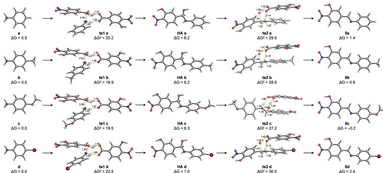
Fig. 4 Lowest-energy structures calculated with SMD(CH 3 CN)/M06-2X/6-311+G(2d,p)//PCM(CH 3 CN)/M06-2X/6-31+G(d,p) for the nucleophilic addition of anilines a–d to aldehyde 1 ( ts1 a–d ), the corresponding hemiaminal intermediates ( HA a–d ) and subsequent water elimination ( ts2 a–d ) to yield imines 5a–d . Both elementary steps are catalyzed with the benzoic acid derivative 1' (see the main text). Relative free energies ( \Delta G ) from the separated reactants are given in kcal·mol -1 and distances are given in Angstrom.
