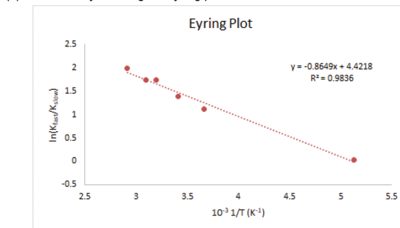
(b) Kinetic analysis using an Eyring plot
