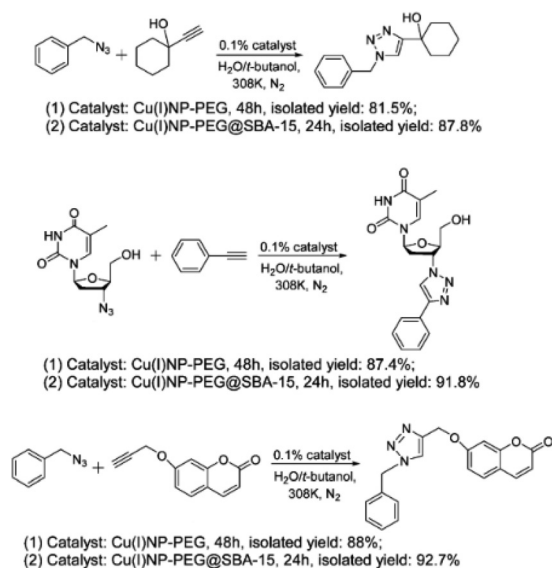
Scheme 10 CuAAC reactions catalysed by supported and unsupported CuNP-PEGs as described in ref. 427. Republished with permission, Copyright 2017 Royal Society of Chemistry.
