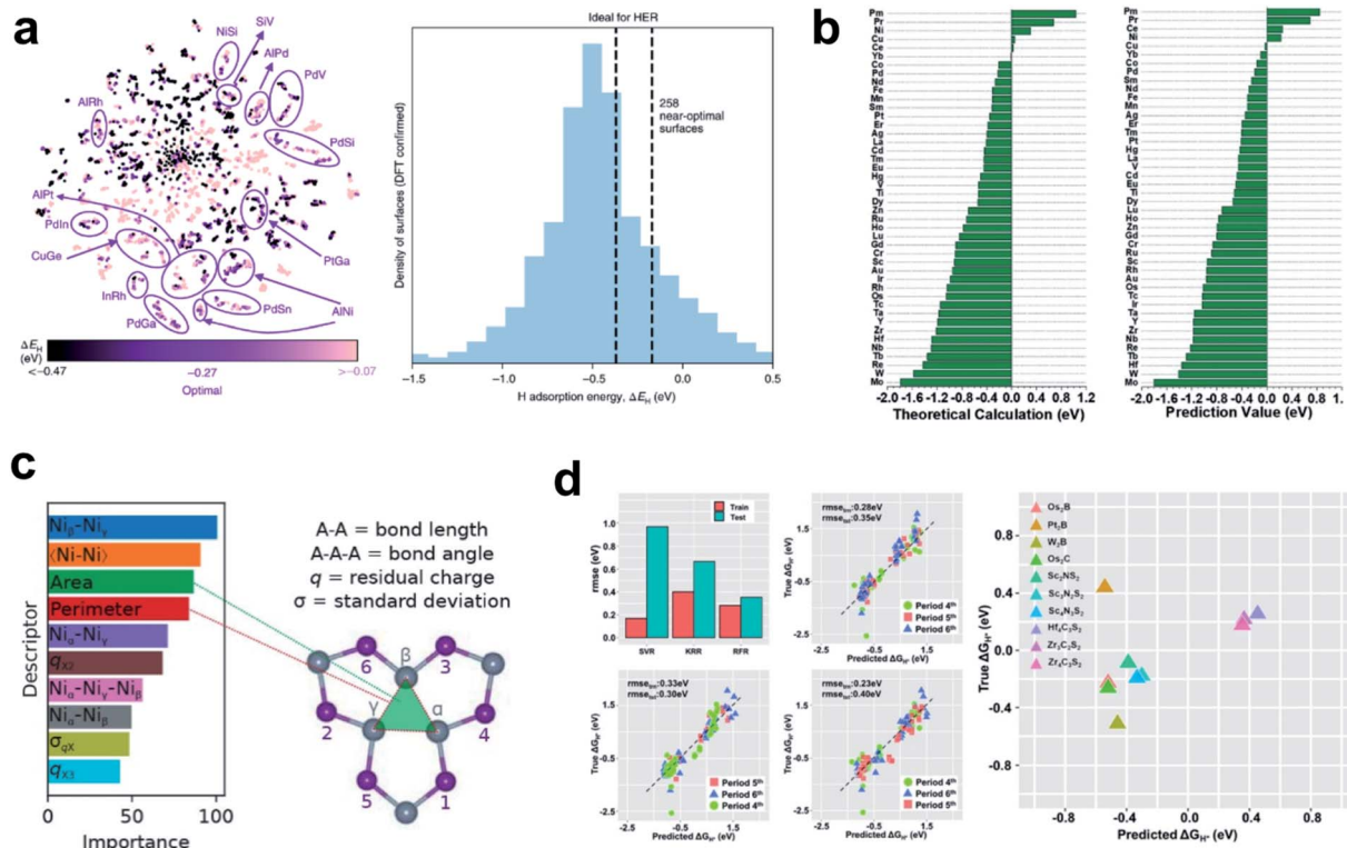
Fig. 4 (a) t-SNE40 visualization of all the adsorption sites simulated using DFT, and normalized distribution of low-coverage \Delta E_{\text{H}} values calculated using DFT. Reproduced from ref. 114. Copyright 2018, Wiley. (b) Comparison of DFT calculation and (b) machine-learning predictions of 2H adsorption energies. Reproduced from ref. 116. Copyright 2019, Wiley. (c) Relative importance of descriptors calculated from the RRF model. Reproduced from ref. 118. Copyright 2018, American Chemical Society. (d) Average root mean square error of SVR, KRR, and RFR obtained using the LOCO CV method. Predicted vs. DFT-calculated \Delta G_{\text{H}^*} of MXenes by using RFR. Reproduced from ref. 117. Copyright 2020, American Chemical Society.
