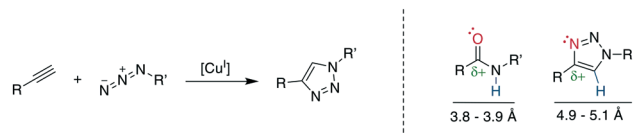
Scheme 32 Left: reaction scheme of the CuI-catalyzed azide–alkyne cycloaddition. Right: comparison of electronic and steric properties of the Z -amide and the 1,4-disubstituted 1,2,3-triazole. Red: H-bond acceptor position, blue: H-bond donor position.
