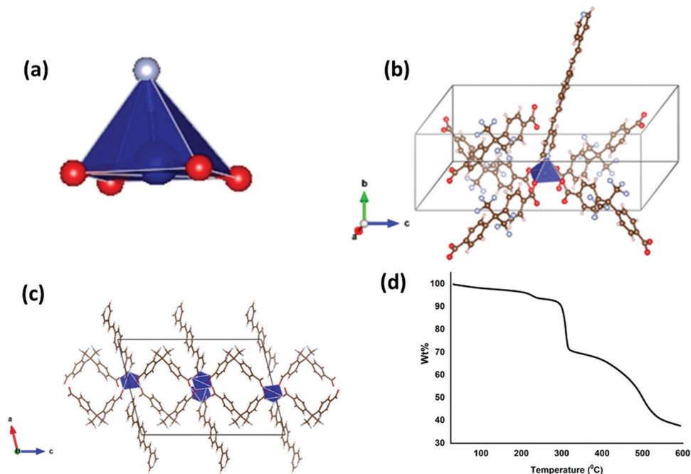
Fig. 1 (a) The SBU unit of the LCo-1 MOF with color code blue: central atom (Co), red: oxygen atoms and indigo blue: nitrogen; (b) complete structure of the SBU with coordinating molecules (bpeb and hfipbb); (c) 2-dimensional structure; and (d) thermogravimetric curve of the LCo-1 MOF.
