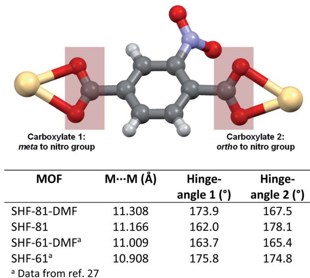
Fig. 3 Carboxylate coordination for \text{NO}_2\text{BDC}^{2-} to consecutive Cd centres in the framework SHF-81 . Analogous coordination is found for \text{NH}_2\text{BDC}^{2-} to consecutive In centres in the framework SHF-61 . Tabulated hinge angles at the two carboxylate groups ( meta and ortho to the ring substituent) are defined as the angle \text{M}\cdots(\text{OO centroid})\cdots(\text{C}_6 \text{ ring centroid}) . Where disorder of the carboxylate group has been modelled, the angles refer to the major component of the model. All single-crystal structures at 100 K (except SHF-61 at 105 K).
