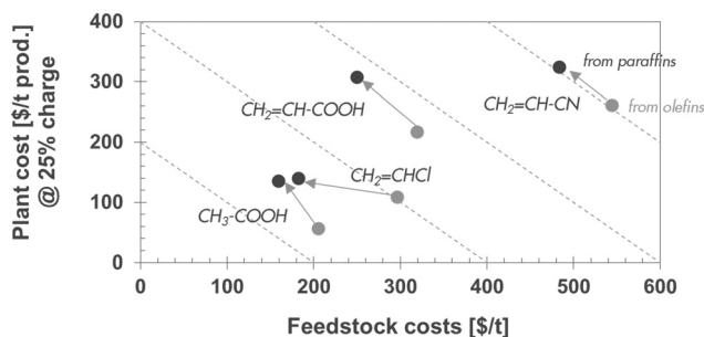
Fig. 3 Challenges in using natural gas. Top: thermodynamic limitation to yields in direct conversion of CH 4 (the acronyms are explained in the appendix). 35 Bottom: economic trade-off between feed and plant costs in direct oxidation of alkanes to chemical intermediates (black) vs. conventional olefin conversion (grey) (the diagonal dotted lines of the bottom figure represent the sum of feed cost and plant cost, the lion's share of the total manufacturing cost). 36
