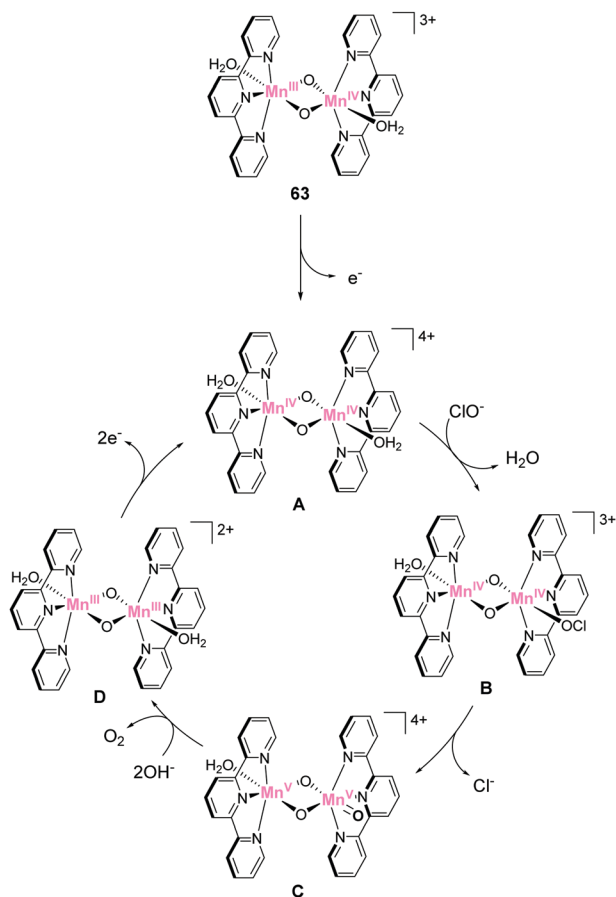
Fig. 28 Plausible catalytic pathway for water oxidation mediated by the bis( \mu -O)-bridged dinuclear manganese complex 63 .
