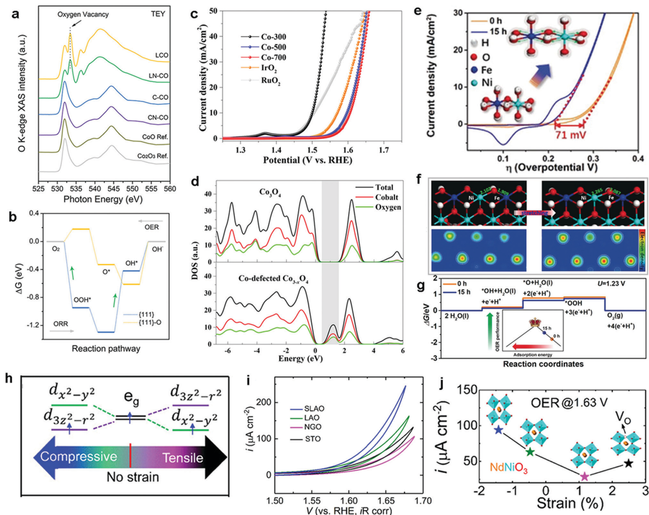
Fig. 12 (a) O K-edge soft XAS spectra of L-CO, LN-CO, C-CO, and CN-CO and CoO and Co 3 O 4 as references. (b) Calculated free energy profiles for the OER/ORR on {111} planes before and after the insertion of oxygen vacancies (green arrow = RDS). Reproduced with permission from ref. 236. Copyright 2019 Wiley VCH. (c) LSV curves of three catalysts and IrO 2 and RuO 2 references for the OER. (d) Computational DOS for Co 3 O 4 and Co-deficient Co 3-x O 4 . Reproduced with permission from ref. 234. Copyright 2018, The American Chemical Society. (e) OER performance of pristine NiFe-LDH and NiFe-LDH after 15 h of ball-milling treatment. (f) Theoretical slab model of NiFe-LDH with and without ball-milling treatment. (g) Computed free energy profiles for (f). Reproduced with permission from ref. 243. Copyright 2019, Wiley VCH. (h) Schematic plots for the strained NNO with e g orbital degeneracy. (i) OER performance for the NNO films grown on different substrates in O 2 -saturated 0.1 M KOH. (j) Plots of current density recorded at 1.63 V of NNO films against the induced strain. Reproduced with permission from ref. 244. Copyright 2019, The American Chemical Society.
