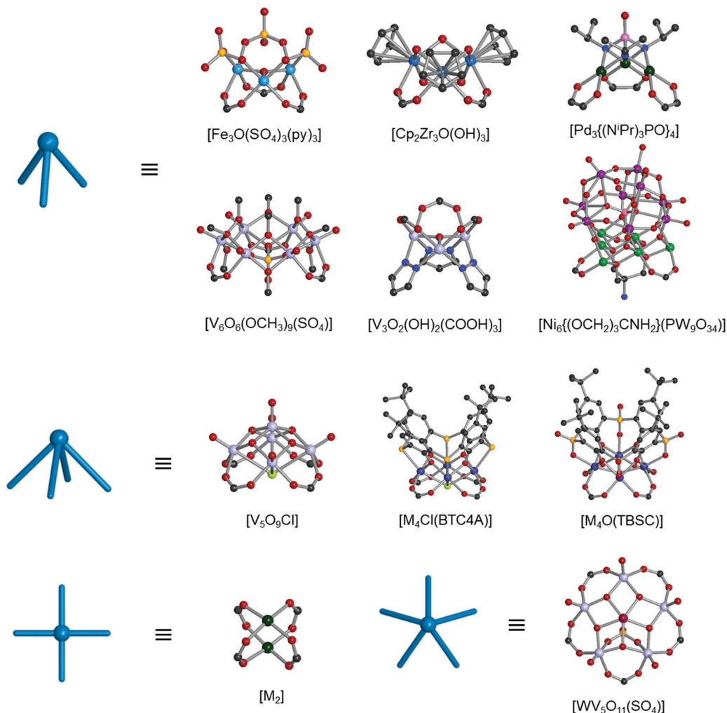
Fig. 2 The list of metal cluster-based SBUs. The first and second rows show the 3-c nodes with 60° coordination angles, [Fe 3 O(SO 4 ) 3 (py) 3 ], [Cp 2 Zr 3 O(OH) 3 ], [Pd 3 {(N i Pr) 3 PO} 4 ], [V 6 O 6 (OCH 3 ) 9 (SO 4 )], [V 3 O 2 (OH) 2 (COOH) 3 ], and [Ni 6 {(OCH 2 ) 3 CNH 2 }(PW 9 O 34 )]. The third row shows the 4-c nodes with 60° coordination angles, [V 5 O 9 Cl], [M 4 Cl(BTC4A)], and [M 4 O(TBSC)]. The fourth row shows the 4-c node with a square-planar coordination geometry, [M 2 ], and the 5-c node with a 60° coordination angle, [WV 5 O 11 (SO 4 )].
