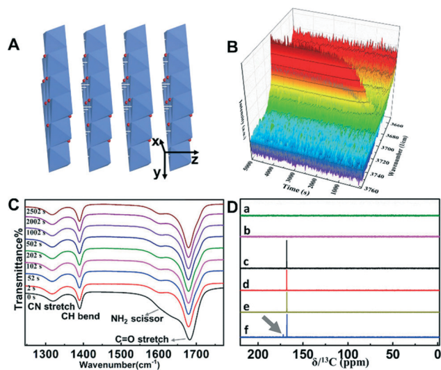
Fig. 4 (A) Atomic structure of Co(OH) 2 , Fe(OH) 2 , Mn(OH) 2 , Zn(OH) 2 , Cu(OH) 2 ·H 2 O and Mg(OH) 2 . (B) Evolution of the typical O–H stretching mode of the Mg–OH groups over time. (C) FTIR spectra of the reaction process after introducing NH 3 into the formamide aqueous solution containing MgCl 2 in the 1000–2000 cm -1 region. (D) 13 C NMR spectra of (a) pure water after introducing NH 3 , (b) aqueous solution containing MgCl 2 after introducing NH 3 , (c) pure formamide aqueous solution, (d) formamide aqueous solution containing MgCl 2 , (e) formamide aqueous solution after introducing NH 3 without MgCl 2 and (f) formamide aqueous solution containing MgCl 2 after introducing NH 3 .
