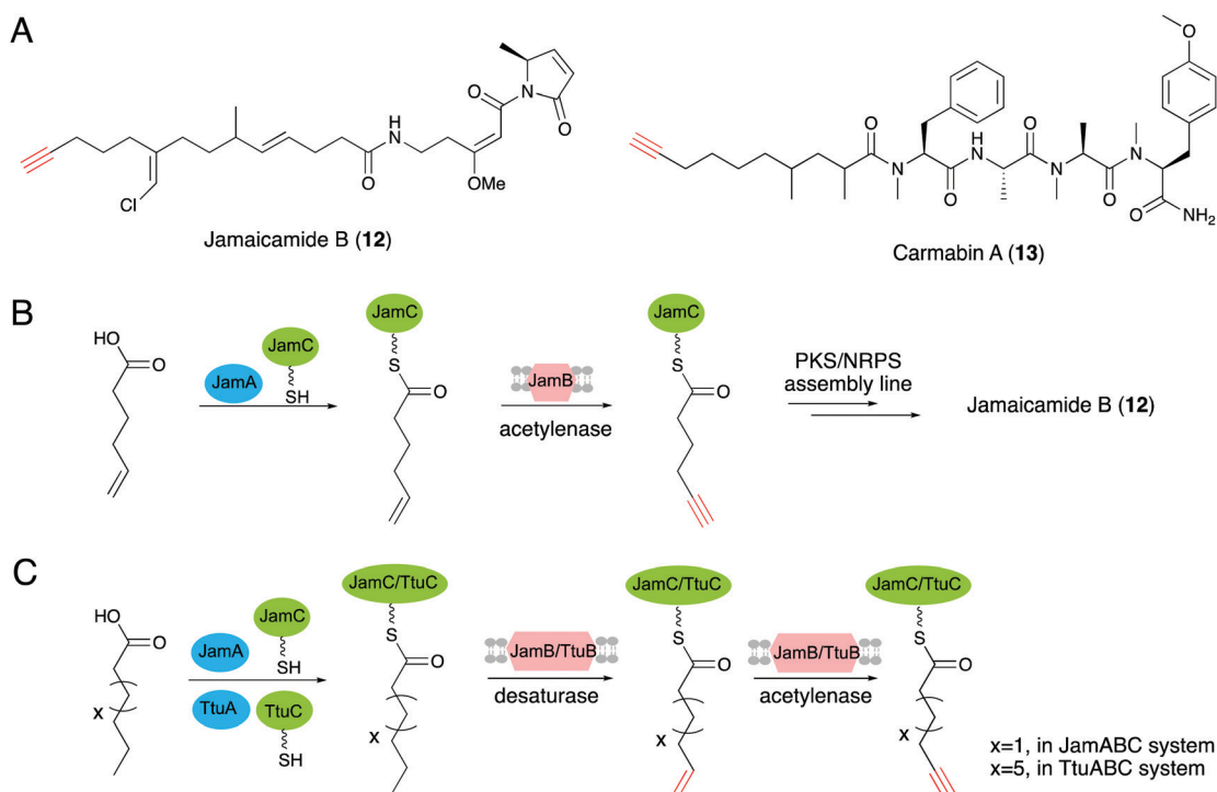
Fig. 6 (A) Structures of 12 and 13 . (B) The biosynthetic pathway for the C 6 alkyne moiety generation and incorporation into jamaicamide B. (C) Terminal alkyne biosynthetic pathways of JamABC and TtuABC that modify C 6 and C 10 fatty acids, respectively.
