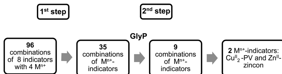
Fig. 3 Two-step screening procedure for the identification of \text{Cu}^{II} -PV and \text{Zn}^{II} -zincon as metal-based GlyP probes.
