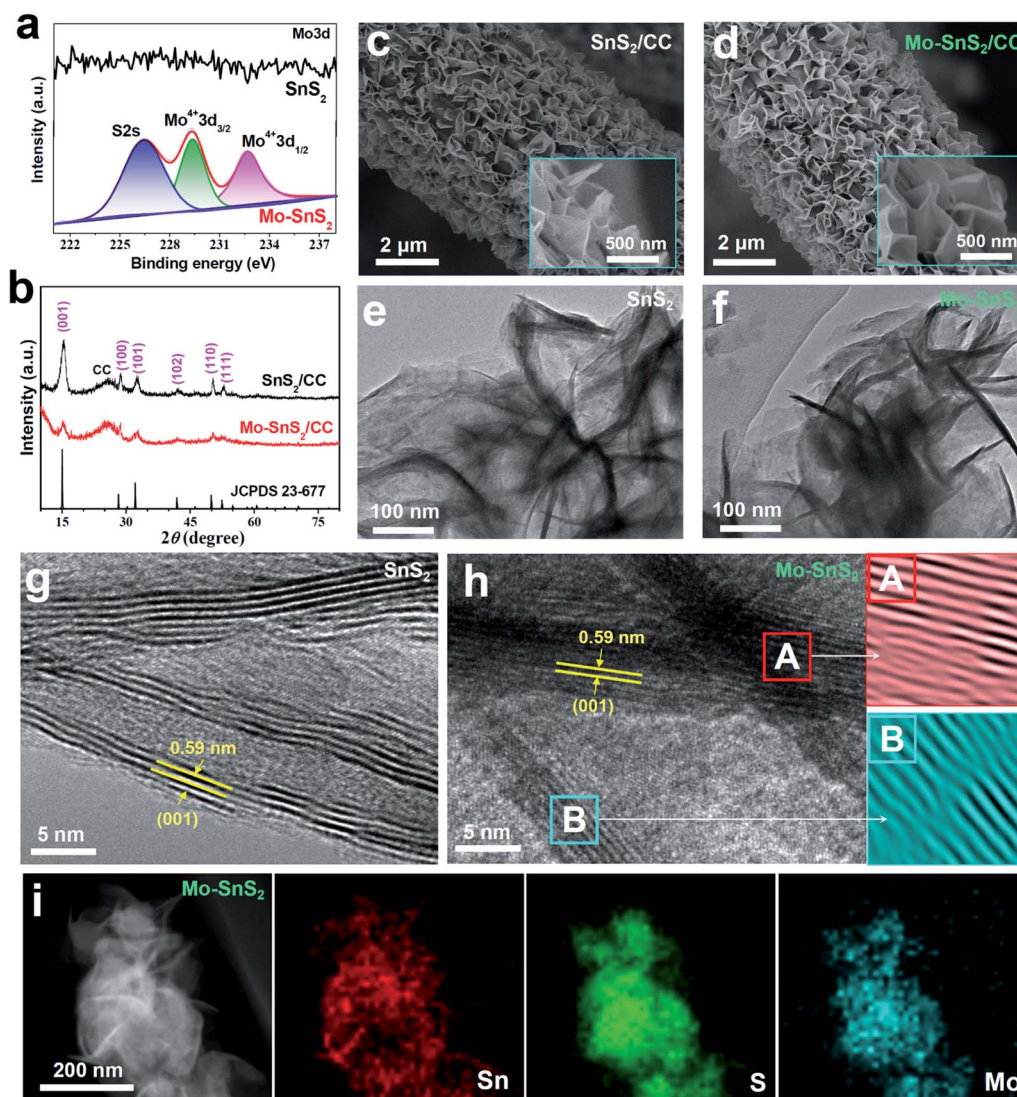
Fig. 1 (a) XPS Mo3d spectrum of SnS 2 and Mo-SnS 2 nanosheets scraped from CC. (b) XRD patterns for SnS 2 /CC and Mo-SnS 2 /CC. (c and d) SEM images of (c) SnS 2 /CC and (d) Mo-SnS 2 /CC. (e and f) TEM images of (e) SnS 2 and (f) Mo-SnS 2 nanosheets. (g and h) HRTEM images of (g) SnS 2 and (h) Mo-SnS 2 nanosheets (A and B are the corresponding IFFT images recorded from regions A and B in (h)). (i) STEM element mapping images for Mo-SnS 2 nanosheets.
