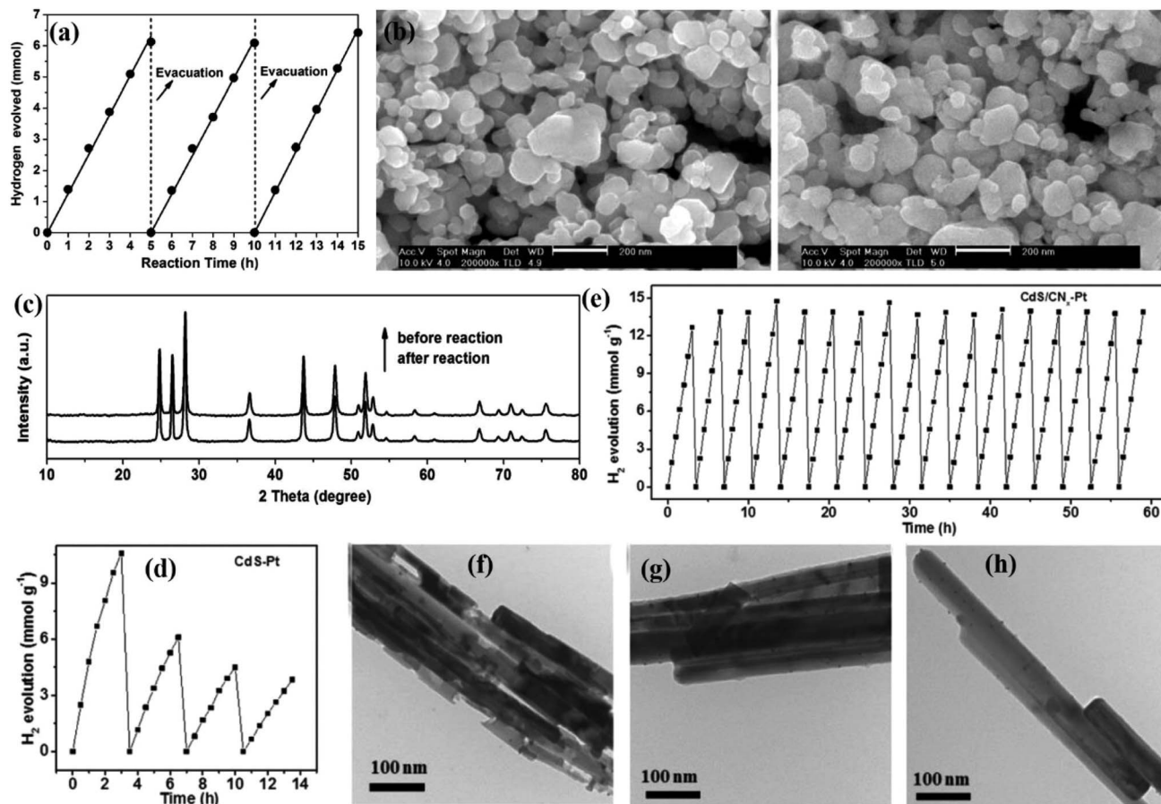
Fig. 2 (a) Time course of \text{H}_2 evolution on 0.9 mol% \text{MoS}_2/\text{CdS} photocatalyst under visible light irradiation; (b) SEM images of 0.9 mol% \text{MoS}_2/\text{CdS} prepared and collected 0.9 mol% \text{MoS}_2/\text{CdS} prepared at 673 K and (c) their XRD patterns. Reprinted with permission from ref. 53. Copyright 2012, Elsevier B.V. The catalytic stability of various photocatalysts for hydrogen production: (d) CdS-Pt and (e) CdS/ \text{CN}_x -Pt, respectively. TEM images of (f) CdS/Pt, (g) CdS-Pt/ \text{CN}_x and (h) CdS/ \text{CN}_x -Pt after cycled \text{H}_2 production. Reprinted with permission from ref. 54. Copyright 2017, Royal Society of Chemistry.
