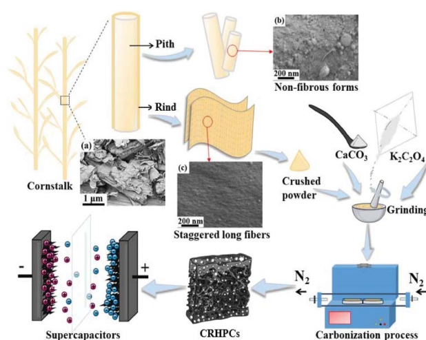
Fig. 1 Schematic fabrication process of the HPCs from cornstalk rind in a one-pot manner (the inserted SEM images are (a) cornstalk (b) cornstalk pith (c) cornstalk rind).
