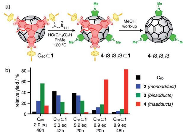
Fig. 4 (a) Cage-templated synthesis of N -methylfulleropyrrolidine trisadducts; (b) relative yields (based on HPLC integration) for unreacted C 60 (black) and Prato adducts 2 (mono, blue), 3 (bis, green) and 4 (tris, red) for control experiment and cage-templated reactions.
