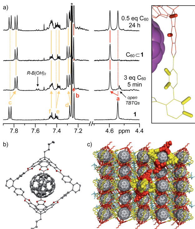
Fig. 3 (a) 1 H-NMR spectra (400 MHz, CDCl 3 , rt) for complexation of 1 with C 60 , (b) ORTEP representation of single-crystal X-ray structure of C 60 < 1 (thermal ellipsoids were set at 50% probability, C = grey, O = red, B = purple, H atoms were omitted for clarity) and (c) packing of C 60 < 1 in the solid state indicating the accessible C 60 surface in the three cage windows.
