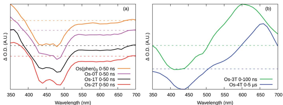
Fig. 8 Transient absorption profiles for (a) [\text{Os}(\text{phen})_3](\text{PF}_6)_2 , Os-0T–Os-2T, and (b) Os-3T and Os-4T, showing the indicated integration slices. \Delta\text{OD} = 0 is indicated by the dashed line of the corresponding color.
