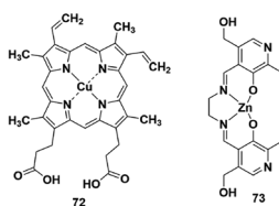
Fig. 13 Representative fluorescent probes based on the coordinative-based approach.
