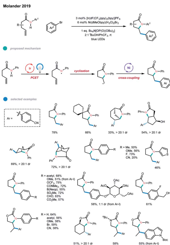
Scheme 11 Cascade amidarylation of unactivated olefins via merging photoredox PCET with nickel catalysis.
