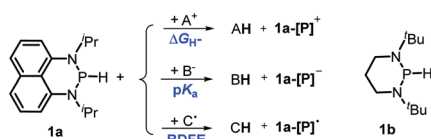
Scheme 2 P–H reagents 1a and 1b serving as diverse hydrogen donors. \text{A}^+ , \text{B}^- and \text{C}^+ are the hydride, proton and hydrogen atom acceptors, respectively.
