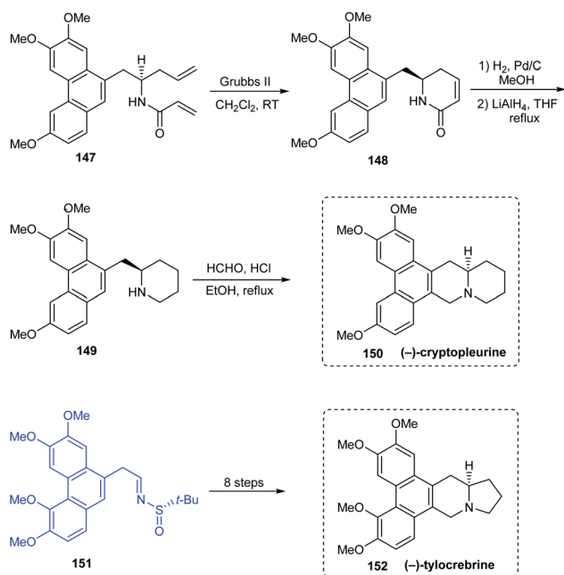
Scheme 26 Asymmetric total synthesis of (-)-tylocrebrine and (-)-cryptopleurine.
