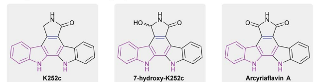
Scheme 4 Phosphoric acid-catalyzed [4 + 2] benzannulation to synthesize carbazoles and indolocarbazoles.
