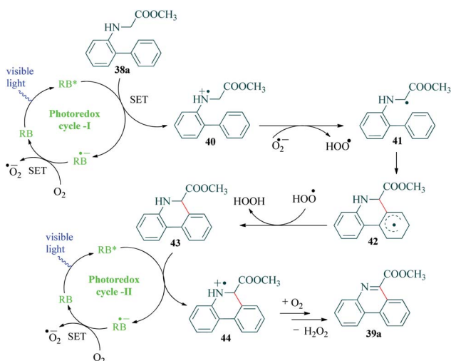
Scheme 12 Photocatalysed conversion of N -biaryl glycine esters to phenanthridines.
