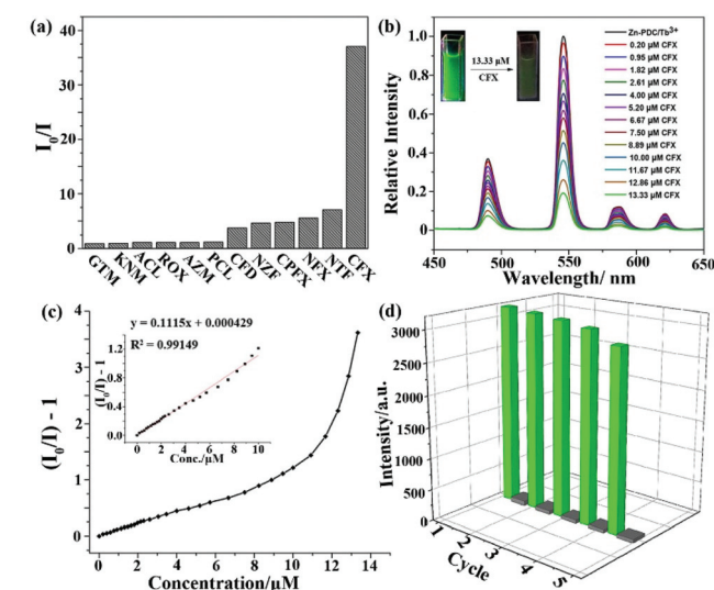
Fig. 12 (a) Luminescence quenching efficiencies of Zn-PDC/Tb 3+ at 546 nm toward different antibiotics. (b) Emission peaks, (c) Stern-Volmer plots and (d) the reusability of Zn-PDC/Tb 3+ toward CFX. Reproduced from ref. 111 with permission from the American Chemical Society.
