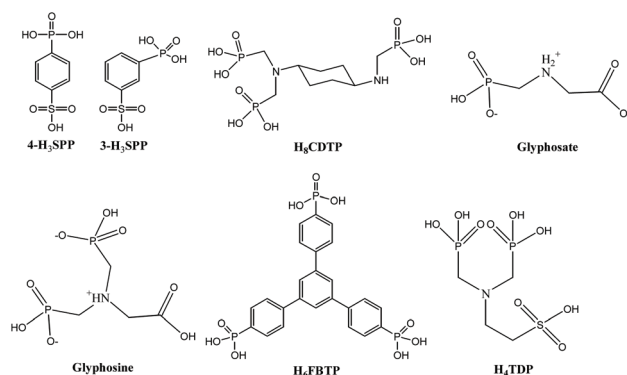
Scheme 4 The organic linkages used in phosphate-based Zr-MOFs.
