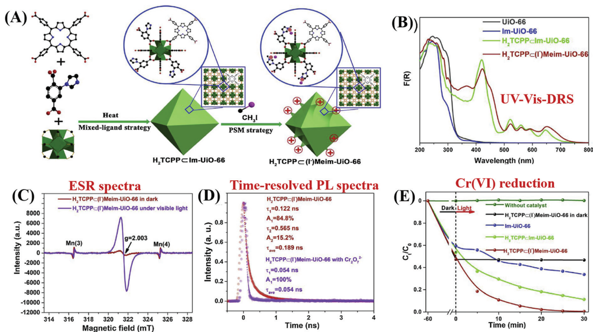
Fig. 36 (A) Schematic processes for the preparation of H_2TCPPC(l^-)Meim-UiO-66 ; (B) UV-vis-DRS of different samples; (C) ESR analyses of H_2TCPPC(l^-)Meim-UiO-66 with Mn as an internal standard; (D) time-resolved PL spectra of H_2TCPPC(l^-)Meim-UiO-66 suspensions with and without the presence of Cr_2O_7^{2-} at an emission wavelength of 650 nm ( \lambda_{ex} = 400 nm); (E) photocatalytic reduction of Cr(VI) by different samples under visible light irradiation. Adapted with permission from ref. 279, © 2019 Elsevier B.V.
