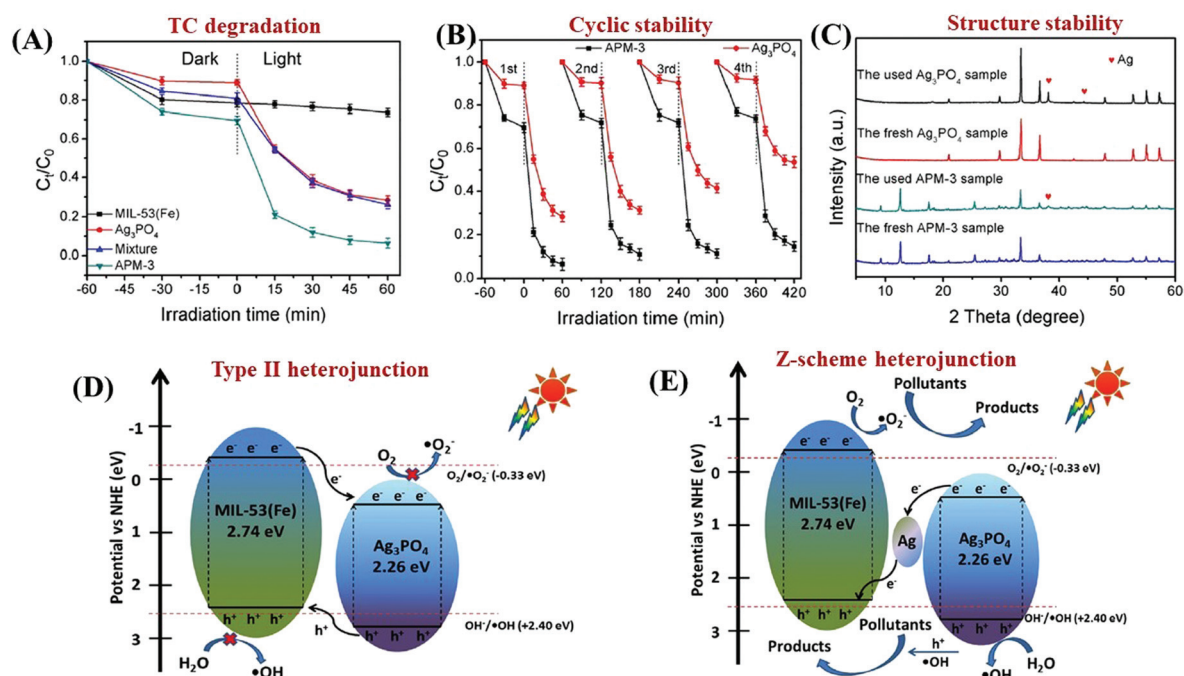
Fig. 28 (A) Photocatalytic degradation of TC by different samples under visible light irradiation; (B) cycling stability of Ag 3 PO 4 and Ag 3 PO 4 /MIL-53 (Fe) composites for photocatalytic degradation of TC; (C) XRD patterns of Ag 3 PO 4 and Ag 3 PO 4 /MIL-53(Fe) under different conditions; proposed mechanism for charge separation over Ag 3 PO 4 /MIL-53(Fe); (D) Traditional Type II heterojunction and (E) Z-scheme heterojunction. Adapted with permission from ref. 165, © 2018 Elsevier B.V.
