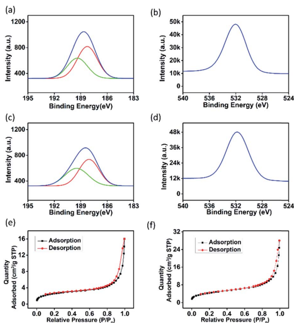
Fig. 5 (a) B 1s XPS spectrum and (b) O 1s spectrum of bulk boron, (c) B 1s XPS spectrum and (d) O 1s spectrum of the exfoliated boron nanostructure; nitrogen adsorption–desorption characterization of (e) bulk boron and (f) exfoliated boron nanostructures.
