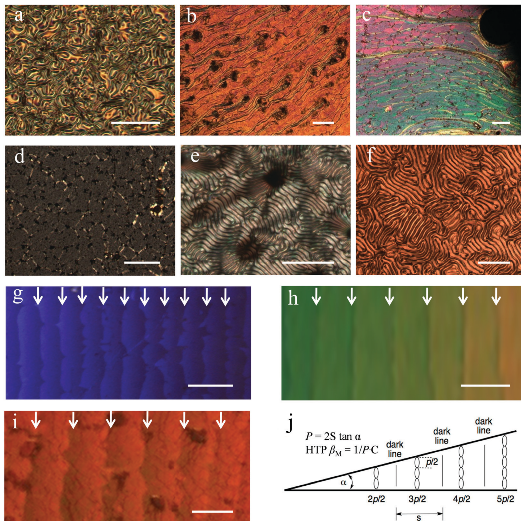
Fig. 2 Optical polarizing microscopy (OPM) micrographs of mesogen L1 doped with (crossed polarizer) (a) 3.5 wt% ChirAuLC1 ( \times 50 \mu\text{m} ) at 25^\circ\text{C} , (b) 6.5 wt% ChirAuLC1 ( \times 100 \mu\text{m} ) at 25^\circ\text{C} , (c) 3.5 wt% ChirAuNP1 ( \times 100 \mu\text{m} ) at 25^\circ\text{C} , (d) 6.5 wt% ChirAuNP1 ( \times 100 \mu\text{m} ) at 25^\circ\text{C} . The induced \text{N}^* phase in 5CB in a homeotropic cell (cell gap = 25 \mu\text{m} ) doped with (e) 3.0 wt% of ChirAuNP1 ( \times 25 \mu\text{m} ) at 30^\circ\text{C} , (f) 3.0 wt% of ChirAuLC1 ( \times 25 \mu\text{m} ) at 30^\circ\text{C} . Images of Grandjean–Cano wedge cells showing Grandjean steps (lines) of the induced \text{N}^* phase in mesogen L1 doped with (g) 5.0 wt% free L2 ( \times 50 \mu\text{m} ) at 25^\circ\text{C} , (h) 3.5 wt% ChirAuNP1 ( \times 50 \mu\text{m} ) at 25^\circ\text{C} , (i) 6.5 wt% ChirAuLC1 ( \times 50 \mu\text{m} ) at 25^\circ\text{C} , (j) Grandjean–Cano wedge cell method to determine the helical pitch ( P ) of the \text{N}^* phase ( S = distance between two disclination lines), and the calculation of the helical twisting power HTP ( \beta_{\text{M}} , a measure for the ability of a chiral dopant to twist a nematic LC phase) followed by the helical pitch measurements, where C is the molar concentration of the chiral additive.
