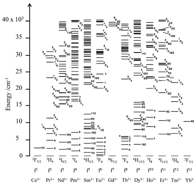
Fig. 4 Energy diagram from the near-infrared to the UV range showing the 2S+1 L J spectroscopic levels of the trivalent lanthanides corresponding to the open-shell 4f n (n = 1–13) electronic configurations. Adapted from ref. 7.
