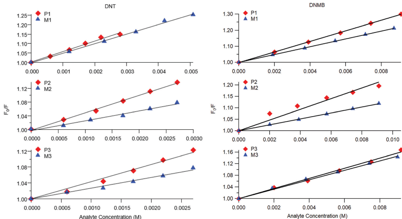
Fig. 3 Representative steady-state Stern–Volmer plots for poly(dendrimer)s P1–3 (red diamonds) and corresponding monomer M1–3 (blue triangles) with DNT (left) and DNMB (right).
