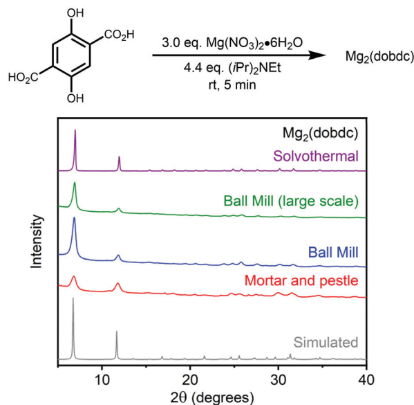
Fig. 3 Powder X-ray diffraction (PXRD) patterns ( \lambda = 1.5406 Å) of \text{Mg}_2(\text{dobdc}) prepared under mechanochemical conditions with a mortar and pestle (red) or ball mill (blue, green) and \text{Mg}_2(\text{dobdc}) prepared under standard solvothermal conditions (purple). 52 The simulated pattern based on the previously reported single-crystal X-ray diffraction structure of the isostructural framework \text{Zn}_2(\text{dobdc}) is included for reference (gray). 53
