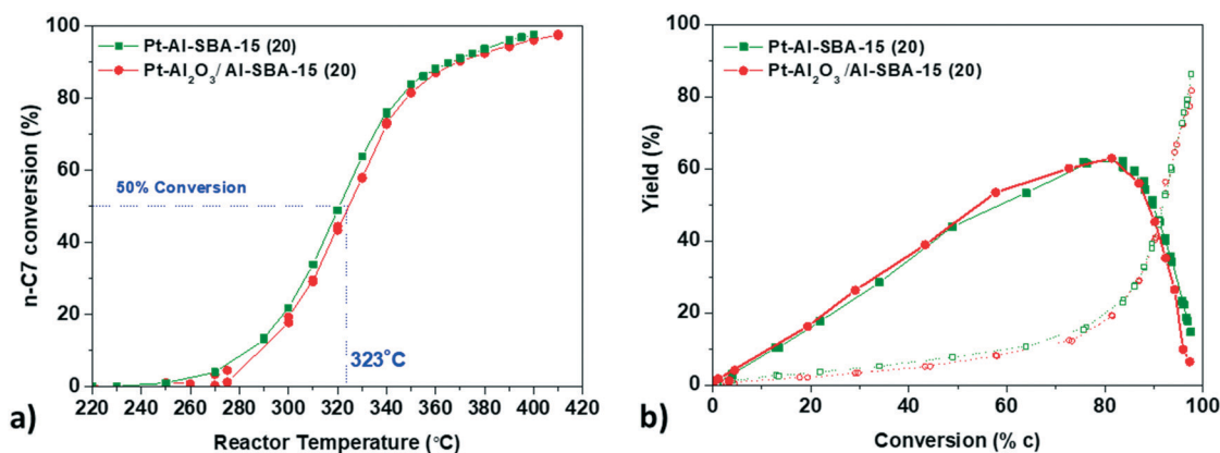
Fig. 3 a. Conversion profile of n -heptane against temperature for Pt-Al-SBA-15 (green squares), Pt-γ-Al 2 O 3 /Al-SBA-15 (red circles) b. yield of C7 isomers (full symbols) and cracking products (open symbols). Catalysis performed at 10 bar; H 2 / n -C7 = 10/1; WHSV = 2.3 g n-C7 g solid acid h -1 .
