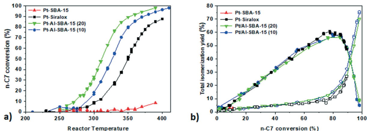
Fig. 2 a. Conversion profile of n -heptane against temperature for Pt-SBA-15 (red triangle); Pt-Al-SBA-15(20) (green triangle); Pt-Al-SBA-15(10) (blue circle) and Pt-ASA (black square) b. yield of isomers against n -C7 conversion for the corresponding catalysts (full symbols) and cracking products (open symbols) catalysis performed at 10 bar; H_2/n\text{-C7} = 10/1 ; WHSV = 1.15 \text{ g}_{n\text{-C7}} \text{ g}_{\text{catalyst}}^{-1} \text{ h}^{-1} .
