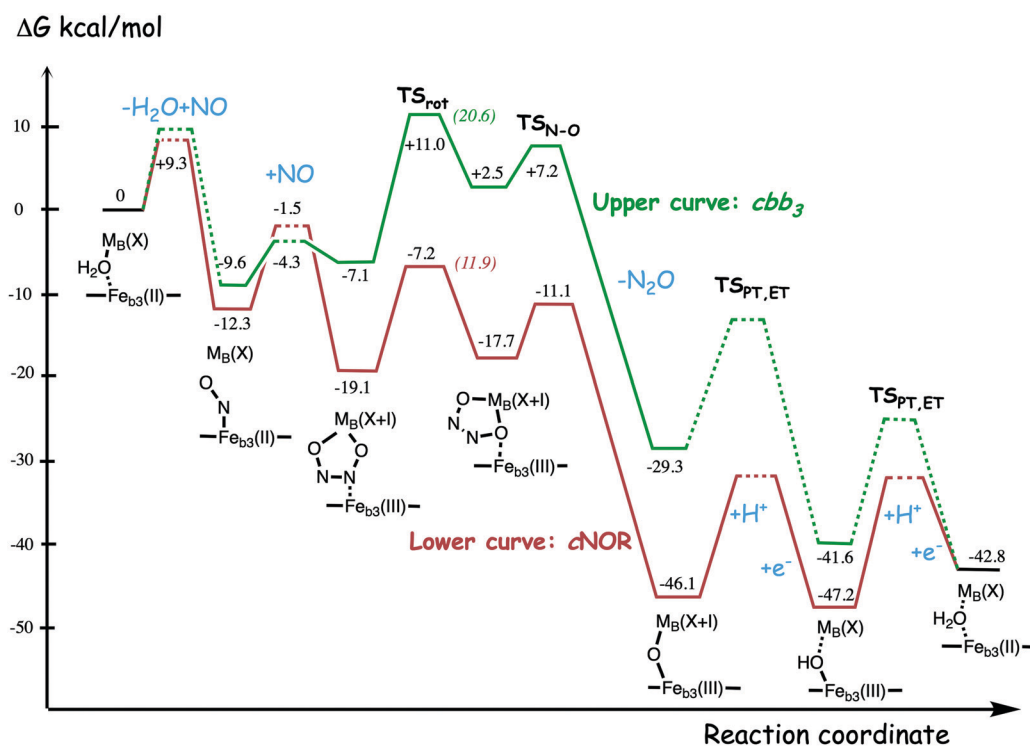
Fig. 24 Calculated free energy profile for one full catalytic cycle of NO reduction in cNOR 12 and in cbb 3 CcO using mechanism I. The notation M_B^{(X)} is used for Fe B (II) in the cNOR case and for Cu B (II) in the cbb 3 case, while the notation M_B^{(X+1)} is used for Fe B (III) and Cu B (III), respectively. The dashed parts of the curves were not studied. The cNOR curve is here calculated relative to the ultimate electron donor cytochrome c, which is different from Fig. 20. The figure is reprinted with permission from ref. 125. Copyright (2020) American Chemical Society.
