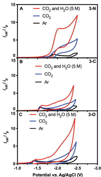
Fig. 1 CV scans of 0.5 mM solutions of 3-N (A), 3-C (B), and 3-O (C) in DMF under argon (black), \text{CO}_2 (blue), and \text{CO}_2 with 5 M \text{H}_2\text{O} (red).
