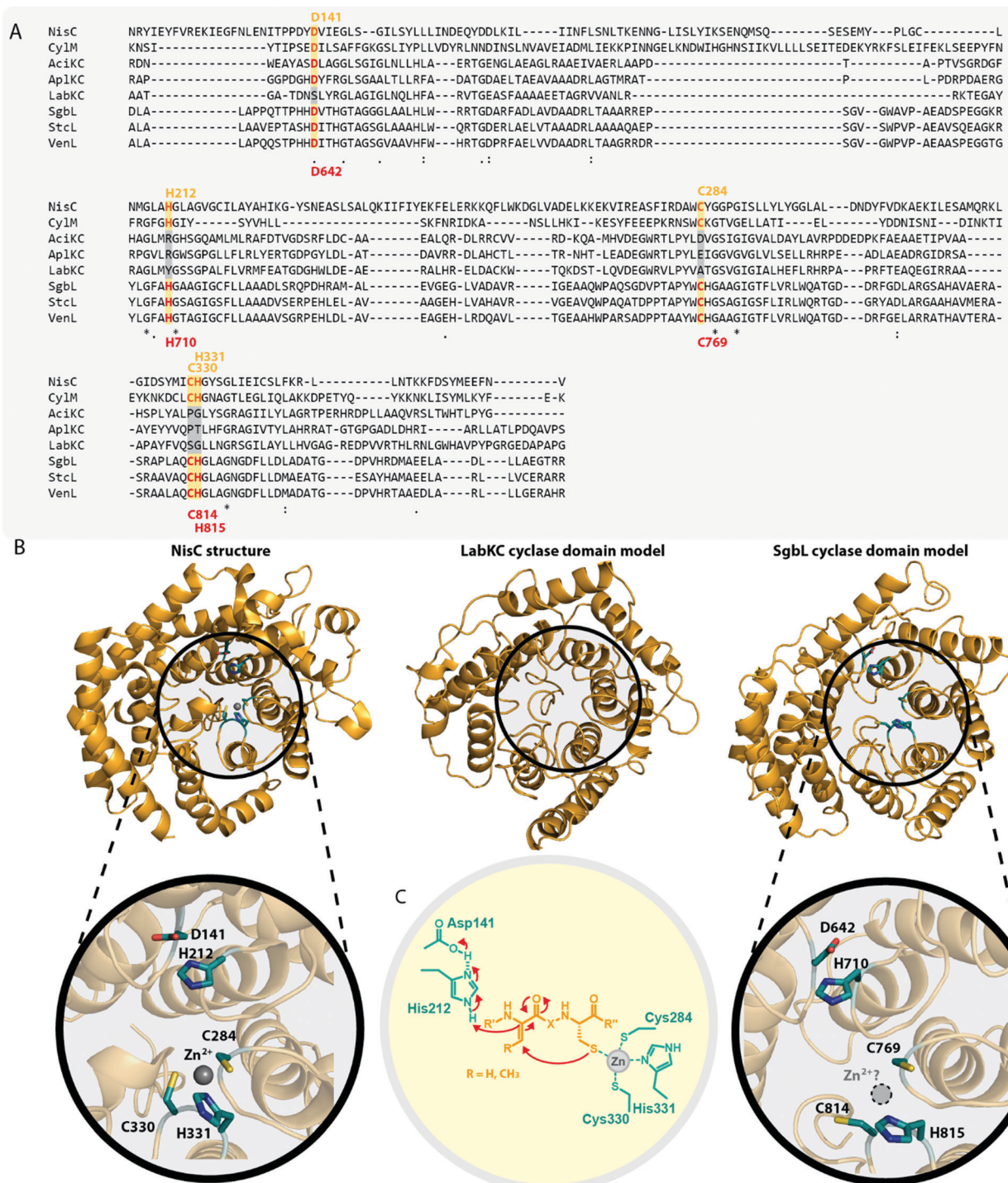
Fig. 7 (A) Excerpt of an alignment of the NisC cyclase (involved in the biosynthesis of the class I lanthipeptide nisin) and the CyIM cyclase domain (involved in the biosynthesis of the class II cytolysin lanthipeptides) with the cyclase domains of exemplary class III (AcIKC, ApIKC, LabKC) and class IV (SgbL, StcL, VenL) lanthipeptide synthetases. Catalytic residues of class I and II cyclases are highlighted in orange, catalytic residues of the class IV cyclase domains in red. Above the alignment, numbering of the catalytic residues of NisC are shown. Below the alignment, numbering of the predicted catalytic residues of SgbL are shown. (B) Comparison of the crystal structure of NisC (PDB code 2G0D) with the Phyre2 models of the LabKC and SgbL cyclase domains. Close ups of the active site of NisC and the predicted active site of the SgbL cyclase domain are shown. Catalytic residues are highlighted in teal. (C) Schematic showing the catalyzed cyclization reaction with the hypothesized 2,5,68,69 functions for the catalytically important residues in NisC.
