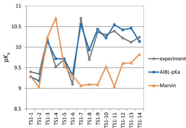
Fig. 5 Relative pK_a values of the primary sulfonamide group across the series TS1-1 to TS1-14. Although Marvin's performance in terms of mean absolute error evaluation is good (0.65), AIBL- pK_a manages to closely match the overall trend in the magnitude of pK_a values across the series.
