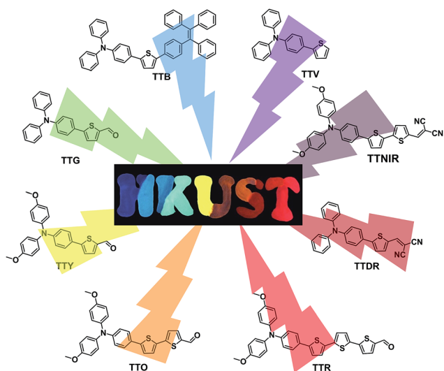
Fig. 1 TPA–thiophene-based AIEgens with widely tunable emissions.
