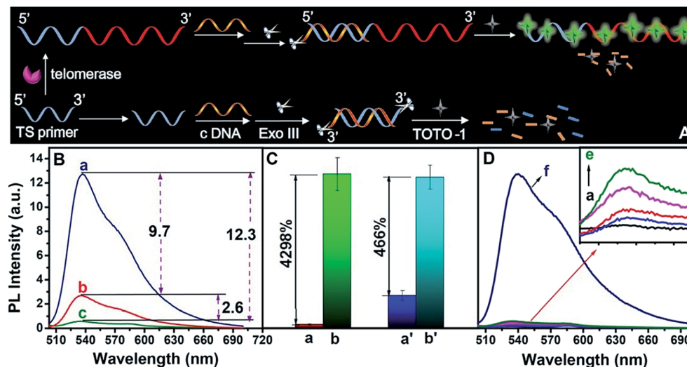
Fig. 4 (A) Scheme of sensing telomerase activity by TOTO-1. (B) PL spectra of TOTO-1/extended-primer/c-DNA/Exo III (a) primer/TOTO-1 (b) and TOTO-1/primer/c-DNA/Exo III (c). (C) PL intensity of TOTO-1 in the presence of primer (a) and elongated primer (b) digested with Exo III; (a') and (b') correspond to (a) and (b) without Exo III. (D) PL spectra of TOTO-1 (a), TOTO-1/primer/Exo III/c-DNA (b), TOTO-1/primer/Exo III/c-DNA in the presence of dNTPs (c), A549 cells (d), dNTPs/Heated A549 cells (e), dNTPs/A549 cells (f); 750 A549 cells per mL and 250 nM TOTO-1 were used.
