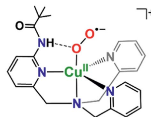
Fig. 9 Intramolecular H-bonding interactions in cupric superoxo complexes, such as in [(\text{PV}\text{TMPA})\text{Cu}^{\text{II}}(\text{O}_2^{\cdot-})]^+ depicted here, result in enhanced reactivity towards phenolic (O–H) substrates. 51,78
