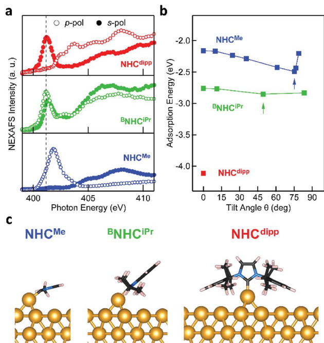
Fig. 2 (a) NEXAFS spectra collected at the N K-edge for \text{NHC}^{\text{Me}} (blue, bottom panel), ^{\text{B}}\text{NHC}^{\text{iPr}} (green), and \text{NHC}^{\text{diPP}} (red) monolayers on Au(111). Each spectrum is measured using X-ray photons with incident electric field in a plane perpendicular to the surface (p-pol, empty circles) or in a plane parallel to the surface (s-pol, filled circles). The N 1s \rightarrow \pi^* -LUMO resonance ( \sim 401 eV, dashed black line) is significantly enhanced in p-pol for \text{NHC}^{\text{Me}} , and in s-pol for \text{NHC}^{\text{diPP}} , indicating a tilt angle \theta \sim 72^\circ and \sim 13^\circ respectively. For ^{\text{B}}\text{NHC}^{\text{iPr}} , both s- and p-pol spectra show the \pi^* -LUMO resonance, yielding \theta \sim 40^\circ . (b) Calculated adsorption energy of \text{NHC}^{\text{Me}} (blue) and ^{\text{B}}\text{NHC}^{\text{iPr}} (green) on an Au adatom as a function of \theta . The adsorption energy of \text{NHC}^{\text{diPP}} (red) is calculated only for \theta = 0^\circ . The arrows indicate the lowest energy structure tilt angles, in good agreement with experimental observations. (c) DFT-optimized minimum energy structure of a single \text{NHC}^{\text{Me}} , ^{\text{B}}\text{NHC}^{\text{iPr}} and \text{NHC}^{\text{diPP}} adsorbed on an Au adatom sitting on a hollow site of an Au(111) slab. These structures are consistent with the experimentally observed tilt angles.
