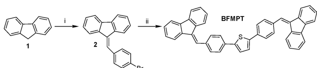
Scheme 1 Synthesis of BFMPT. Reagents and conditions: (i) 4-bromobenzaldehyde, KOH, EtOH, n\text{-Bu}_4\text{NI} , 2 h, reflux, 80%; (ii) 2,5-bis(tri( n -butyl)stannyl)thiophene, \text{Pd}(\text{PPh}_3)_4 (5 mol%), DMF, 80^\circ \text{C} , 6 h, 90%.
