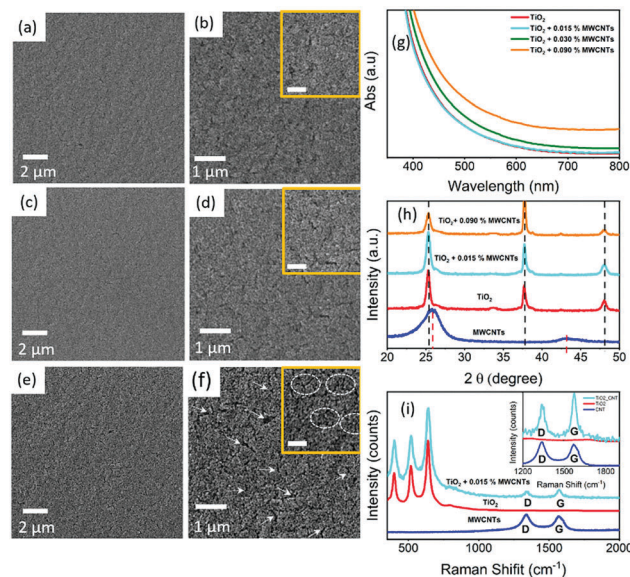
Fig. 2 SEM images of mesoporous \text{TiO}_2 films with different content of MWCNTs: (a and b) 0 \text{ wt}\% ; (c and d) 0.015 \text{ wt}\% and (e and f) 0.030 \text{ wt}\% at different magnifications. The inset of b, d, and f are high-resolution SEM images of corresponding mesoporous films. The presence of deep cracks induced at higher concentrations of the MWCNTs is clearly visible in (f) (white arrows) and the inset (dotted circles highlights a crack zone area). A systematic comparison of the patterns of MWCNTs, bare \text{TiO}_2 and \text{TiO}_2 -MWCNT mesoporous films at different concentrations of MWCNTs: (g) absorption spectra; (h) XRD; (i) Raman spectra, the inset highlights the D and G bands of the MWCNTs and \text{TiO}_2 -MWCNTs.
