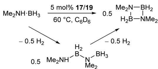
Scheme 12 Dehydrocoupling of \text{Me}_2\text{NH}\cdot\text{BH}_3 catalysed by low coordinate Mn(II) terphenyl complexes. 72
